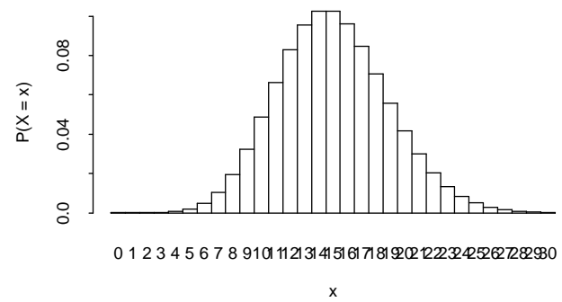
Poisson Prob. Fun., mu=15
